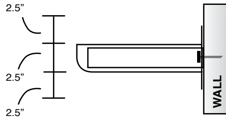
SECTION VIEW
