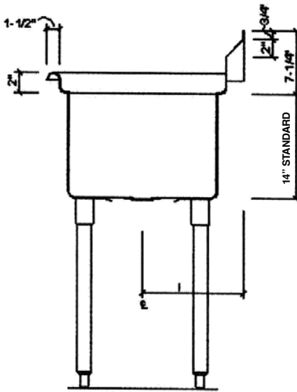
SECTION VIEW
