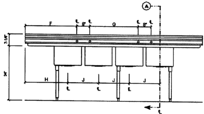
ELEVATION VIEW
