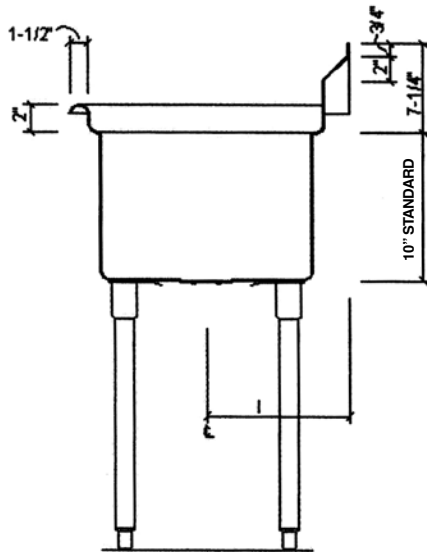
SECTION VIEW
