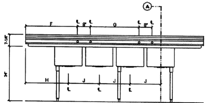
ELEVATION VIEW
