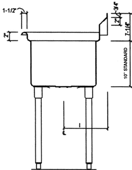
SECTION VIEW
