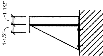
SECTION VIEW
