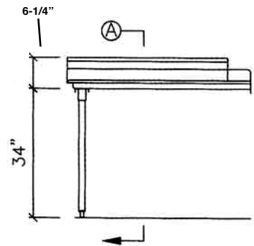
ELEVATION VIEW
