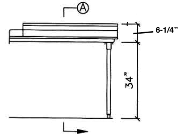
ELEVATION VIEW
