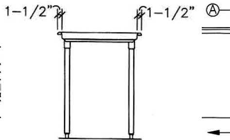
SECTION VIEW
